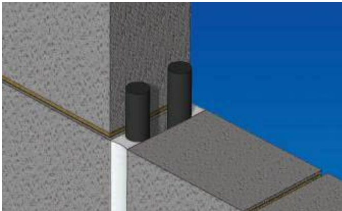
Acrylic Sealant Masonry wall PE backing spacer
